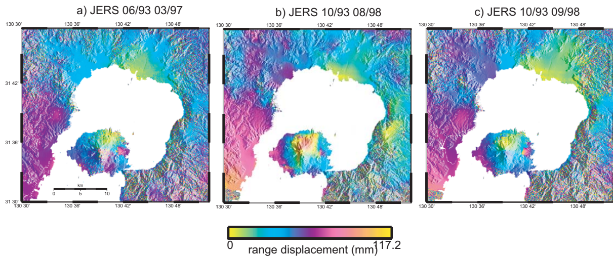
Fig. 2. Recorded differential JERS interferograms over the Aira Caldera encompassing the 1993–1998 period. (a) Interferogram spanning four years from June 1993 to March 1997. (b) Interferogram spanning five years from October 1993 to August 1998. (c) Interferogram spanning five years from October 1993 to September 1998. A complete cycle of phase (purple, blue, yellow) represents a decrease in range of 11.73 cm between the ground surface and the satellite.
